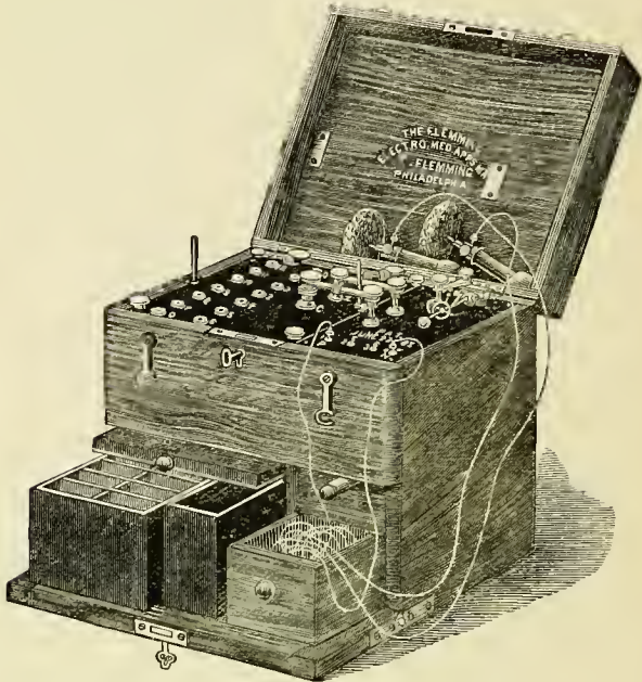
FLEMING'S 30-CELL COMBINATION BATTERY.
